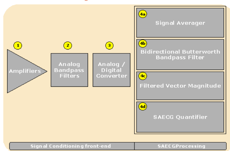
Block Diagram of HRECG Instrument
